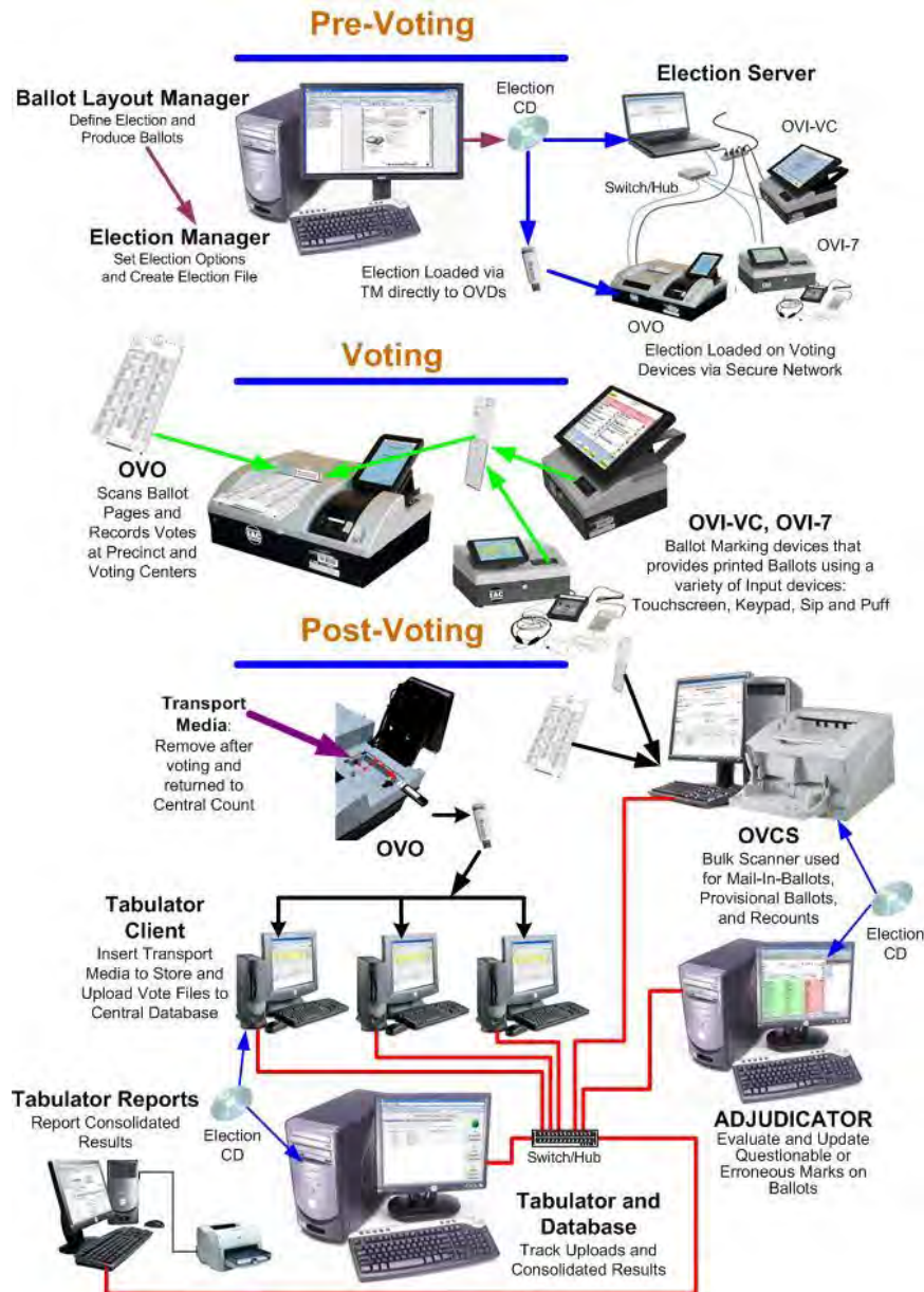
Figure No. 7 System Overview Diagram
