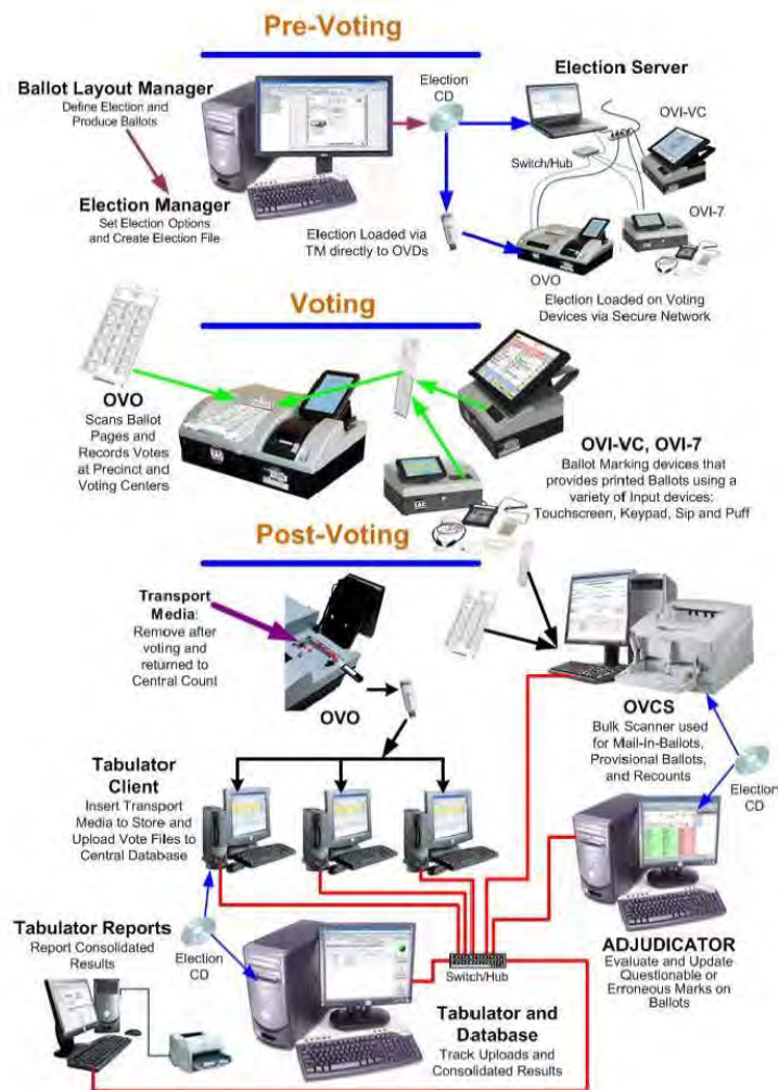
Figure 1-7 System Overview Diagram
