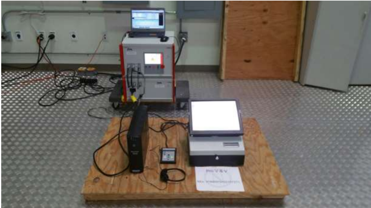
EFT Test Configuration Photograph - OVI-VC
