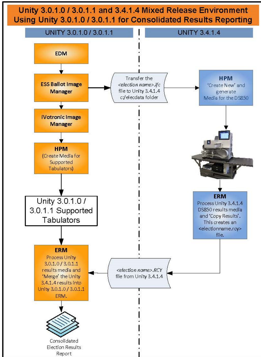
Figure A-1. Unity Bridge Diagram
